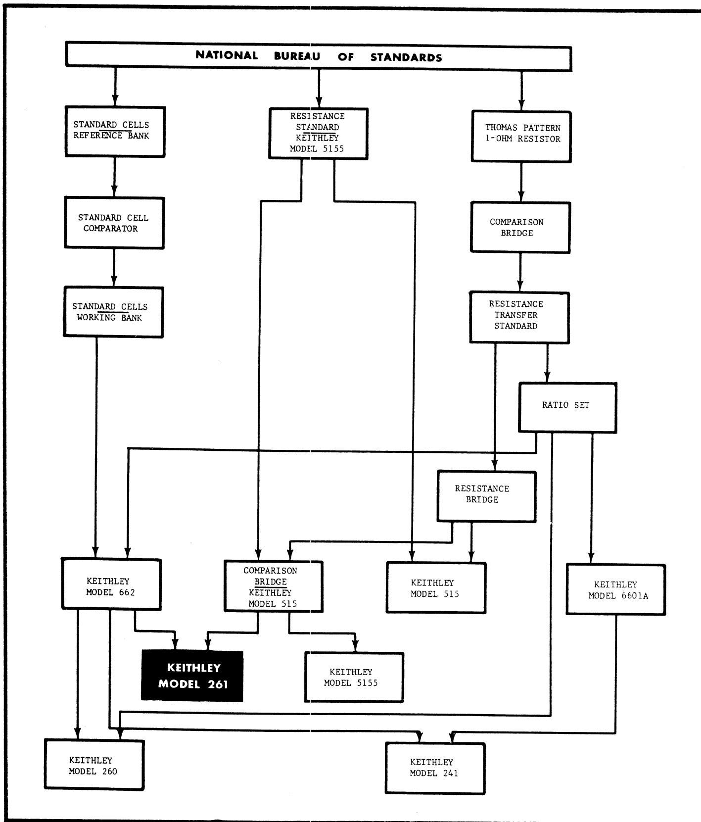
FIGURE 13. Model 261 Traceable Chart to National Bureau of Standards. Other Keithley instruments are also shown.
