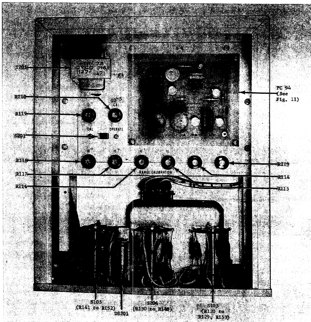
FIGURE 10. Top View of Model 261 Chassis. The front panel is along the bottom of the photograph. Location of components is shown. Refer to Replaceable Parts List for circuit designations.
